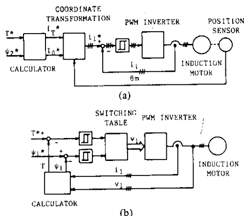
Fig. 1. Comparison of two schemes. (a) Field-oriented control. (b) New proposed scheme.
