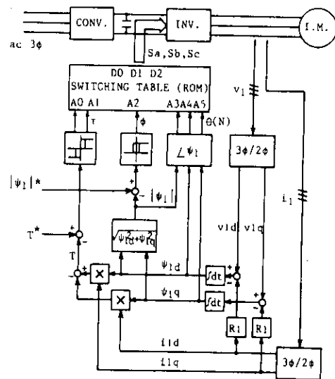
Fig. 8. Block diagram of proposed system.
