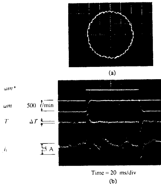
Fig. 9. Experimental results. (a) Locus of \psi_1 at 600 r/min. (b) Velocity step response.
