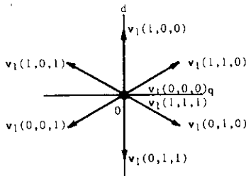
Fig. 4. Instantaneous voltage vectors.
