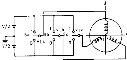
Fig. 3. Schematic diagram of PWM inverter.
