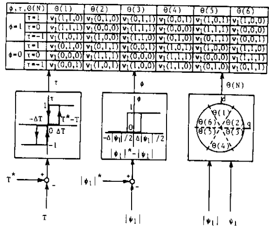
Fig. 7. Optimum switching table and comparators.
