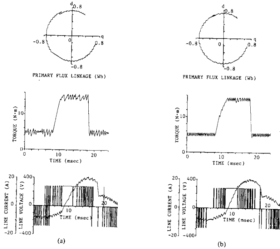
Fig. 10. Simulation results for comparison between schemes. (a) Field-oriented control. (b) Proposed control. (Induction motor parameters: R_1 = 0.5 \Omega ; R_2 = 1.0 \Omega ; L_{11} = 0.105 \text{ H} ; L_{22} = 0.105 \text{ H} ; M = 0.1 \text{ H} ; number of poles = 2; \theta_m = 188.5 \text{ rad/s} ; 1800 r/min; V = 280 \text{ V} ; switching frequency = 2.5 kHz.)
