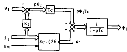
Fig. 12. Improved flux estimator.
